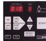
Metal Halide Exposure unit AM-150
